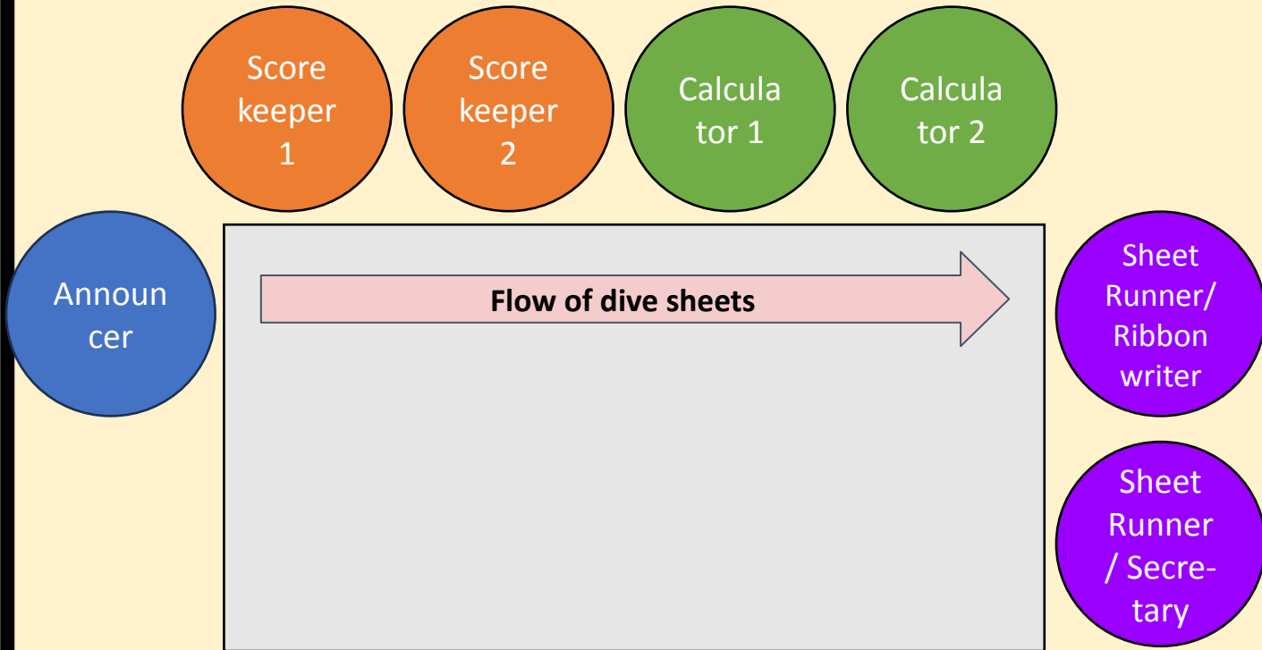
Configuration A
